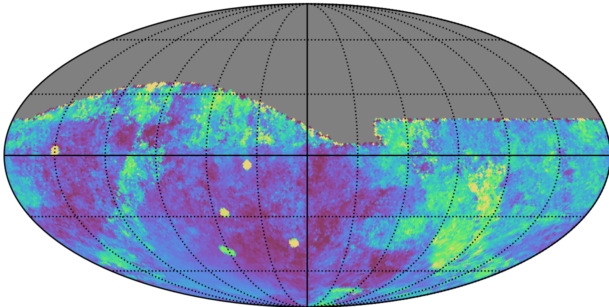
baseline_v2.0_10yrs All sky all bands: Median moonDistance
