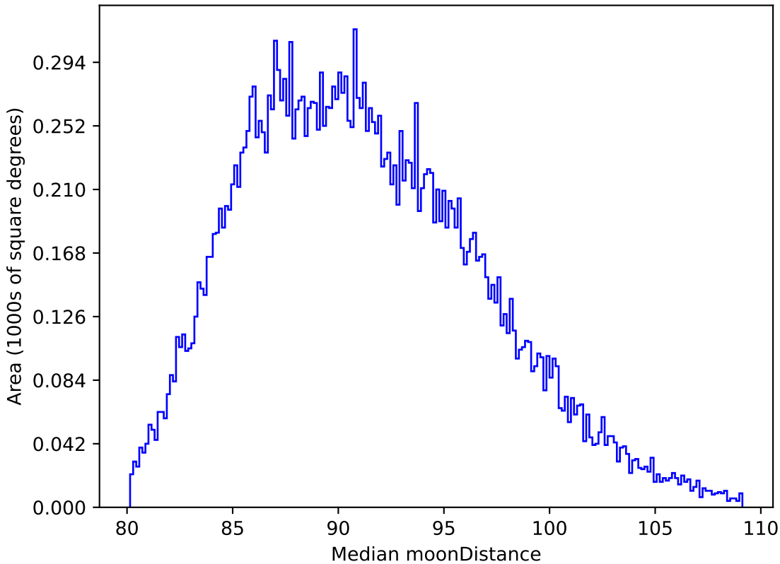
baseline_v2.0_10yrs All sky all bands: Median moonDistance
