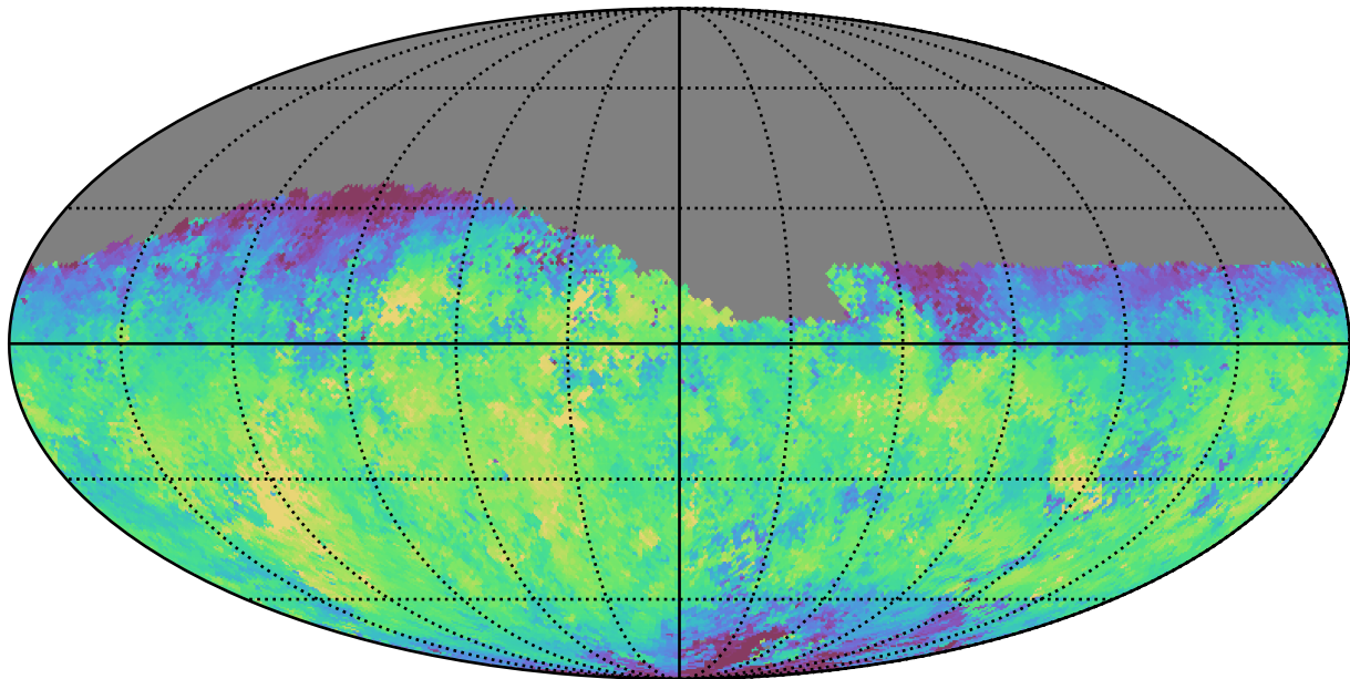
baseline_v2.0_10yrs Yr 1 z band: Median fiveSigmaDepth
