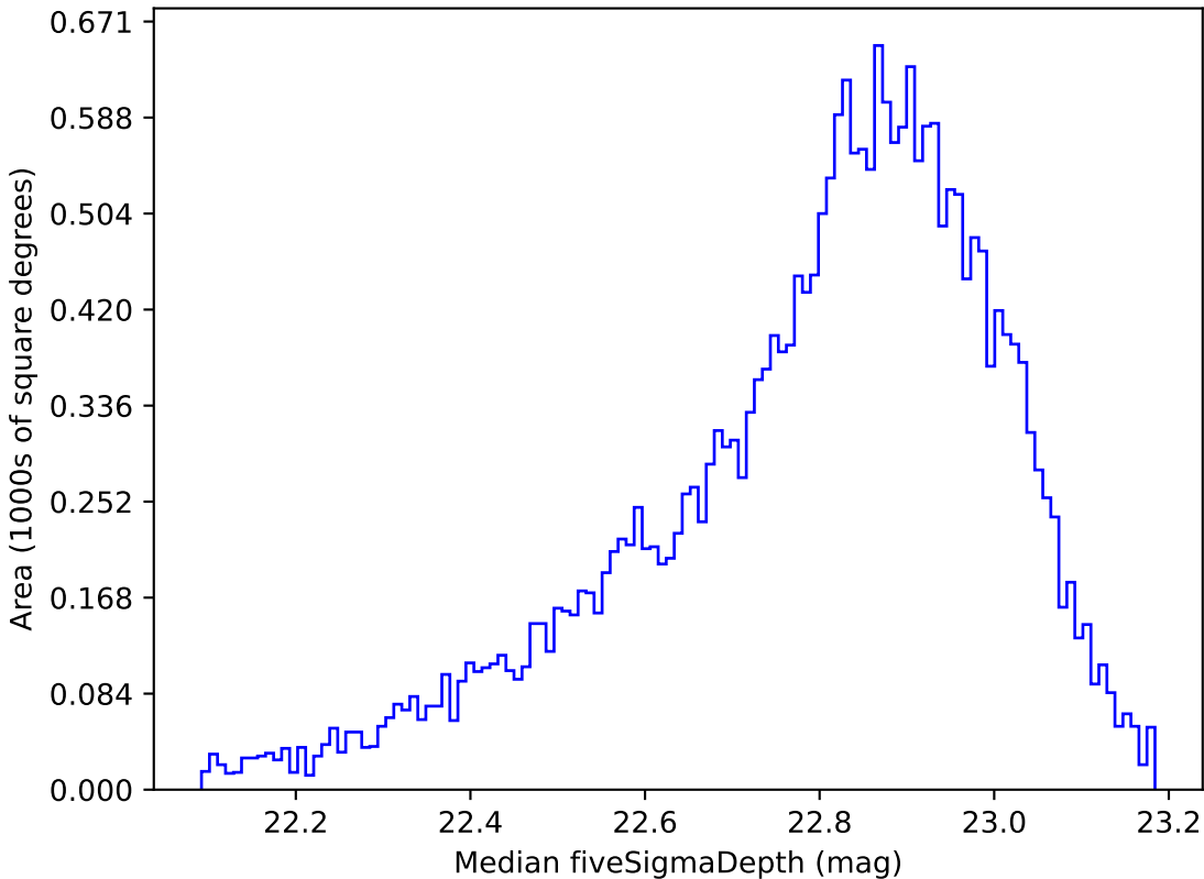
baseline_v2.0_10yrs Yr 1 z band: Median fiveSigmaDepth
