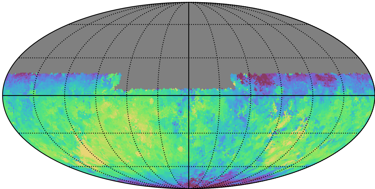
baseline_v2.0_10yrs Yr 1 y band: Median fiveSigmaDepth
