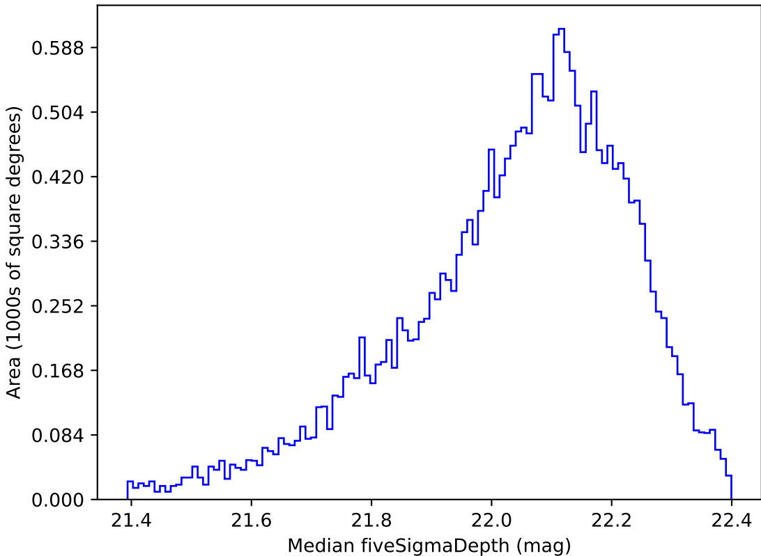
baseline_v2.0_10yrs Yr 1 y band: Median fiveSigmaDepth
