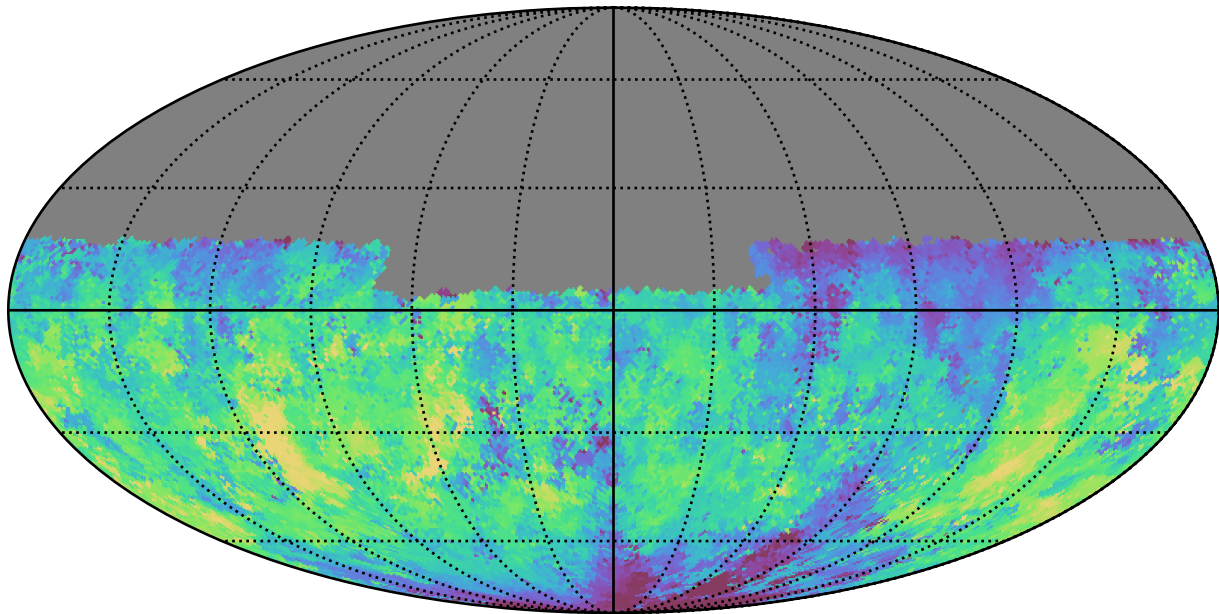
baseline_v2.0_10yrs Yr 1 u band: Median fiveSigmaDepth
