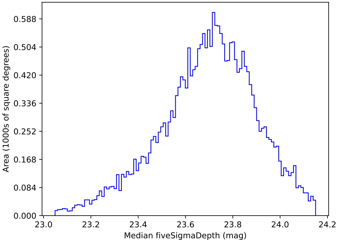
baseline_v2.0_10yrs Yr 1 u band: Median fiveSigmaDepth
