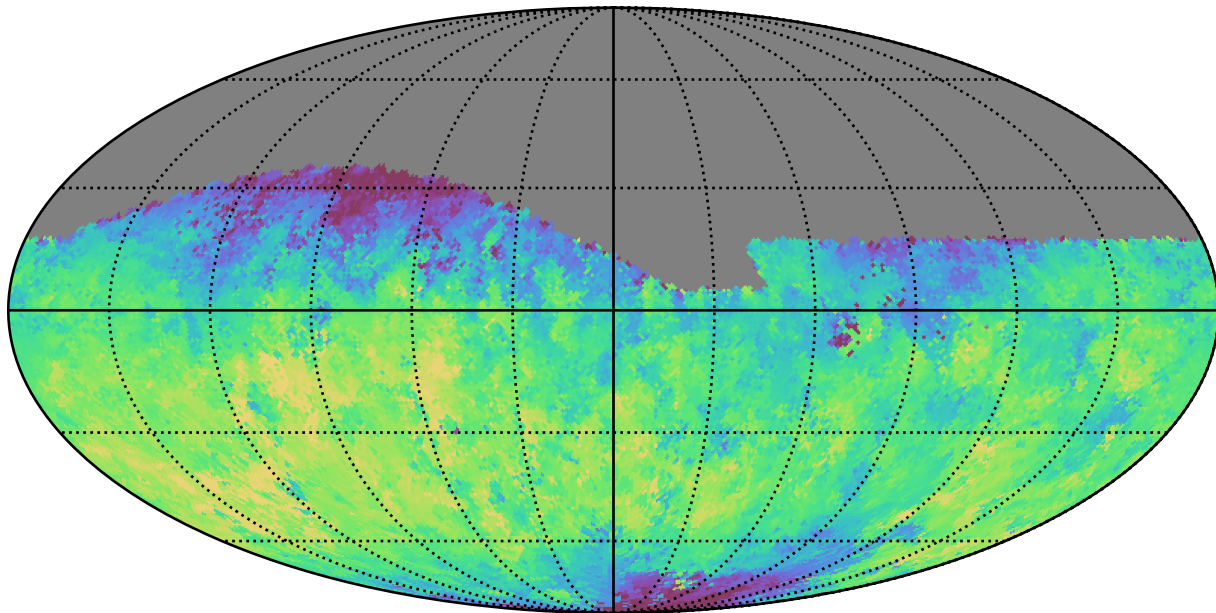
baseline_v2.0_10yrs Yr 1 r band: Median fiveSigmaDepth
