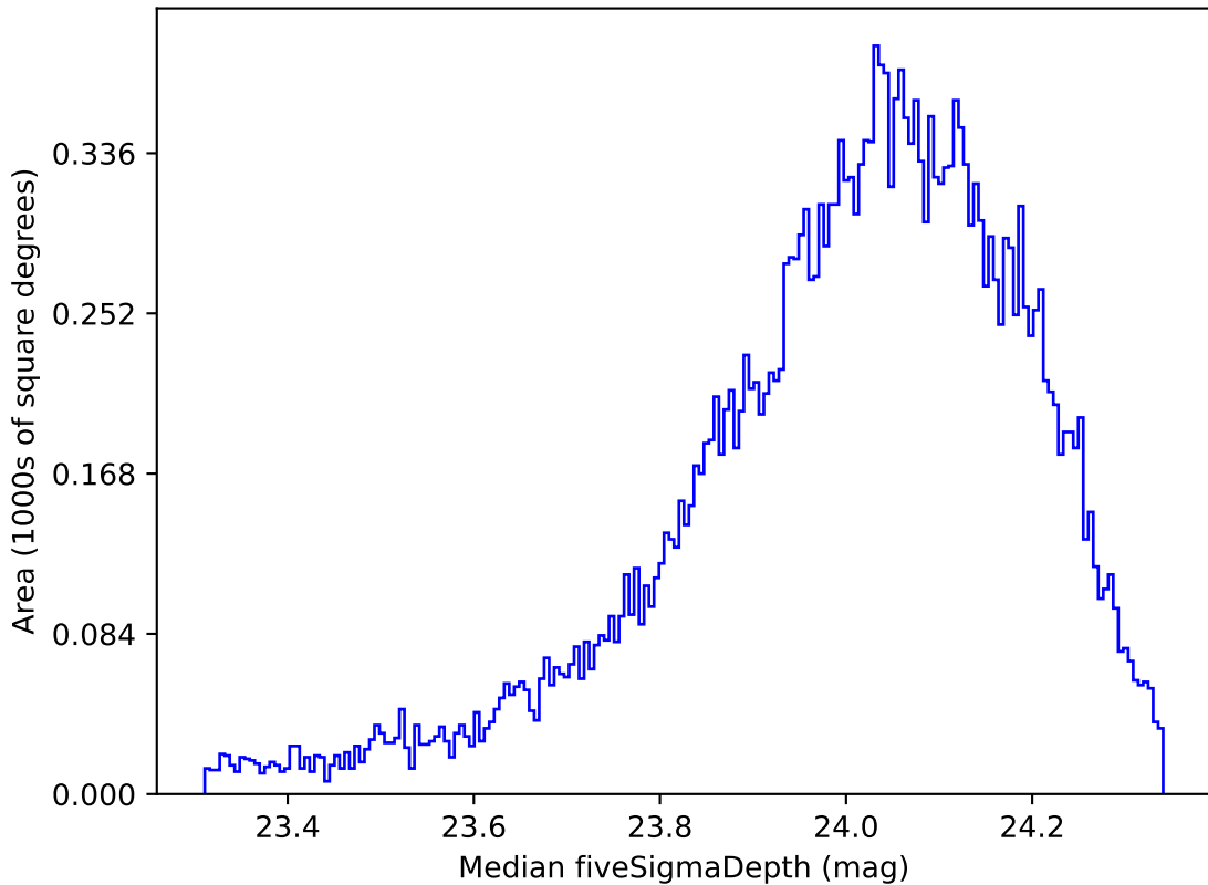
baseline_v2.0_10yrs Yr 1 r band: Median fiveSigmaDepth
