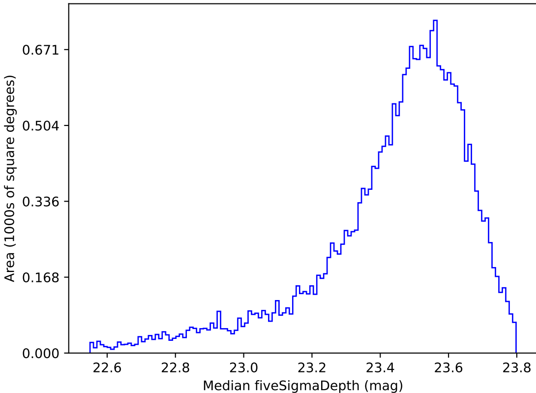
baseline_v2.0_10yrs Yr 1 i band: Median fiveSigmaDepth
