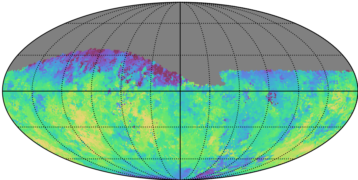
baseline_v2.0_10yrs Yr 1 g band: Median fiveSigmaDepth
