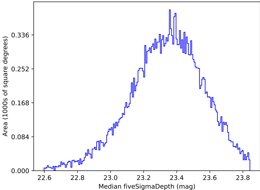
baseline_v2.0_10yrs Yr 1 all bands: Median fiveSigmaDepth
