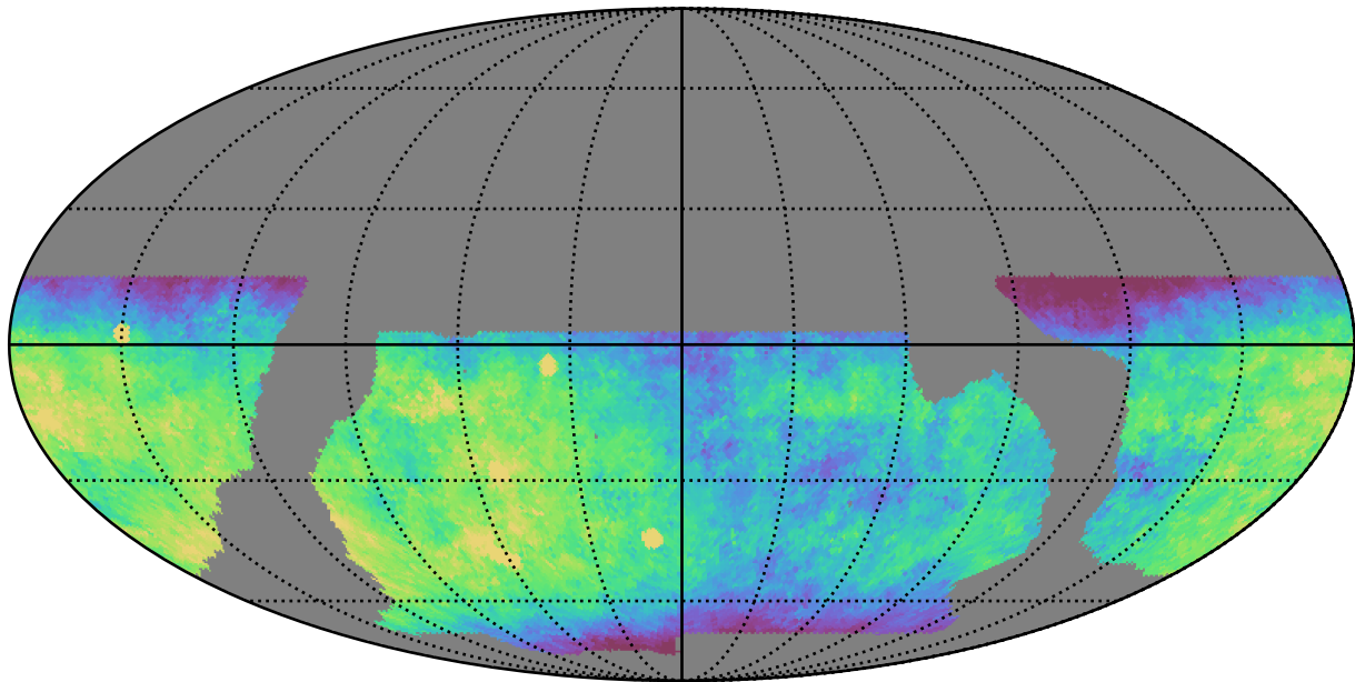
baseline_v2.0_10yrs WFD z band: Median fiveSigmaDepth
