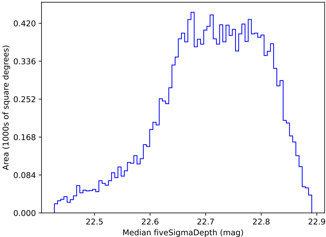
baseline_v2.0_10yrs WFD z band: Median fiveSigmaDepth
