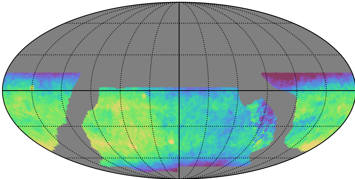
baseline_v2.0_10yrs WFD y band: Median fiveSigmaDepth
