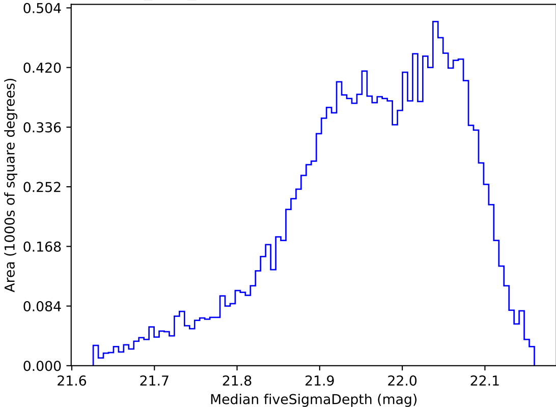
baseline_v2.0_10yrs WFD y band: Median fiveSigmaDepth
