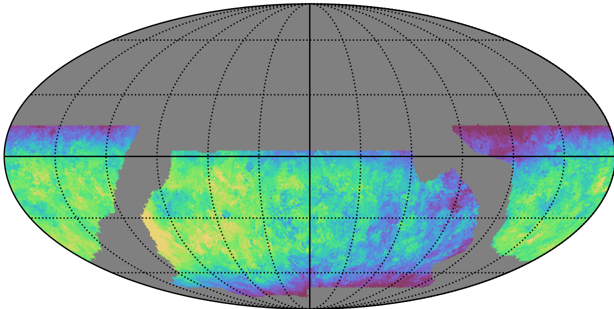
baseline_v2.0_10yrs WFD u band: Median fiveSigmaDepth
