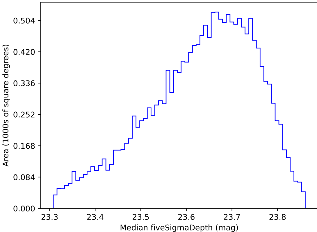
baseline_v2.0_10yrs WFD u band: Median fiveSigmaDepth
