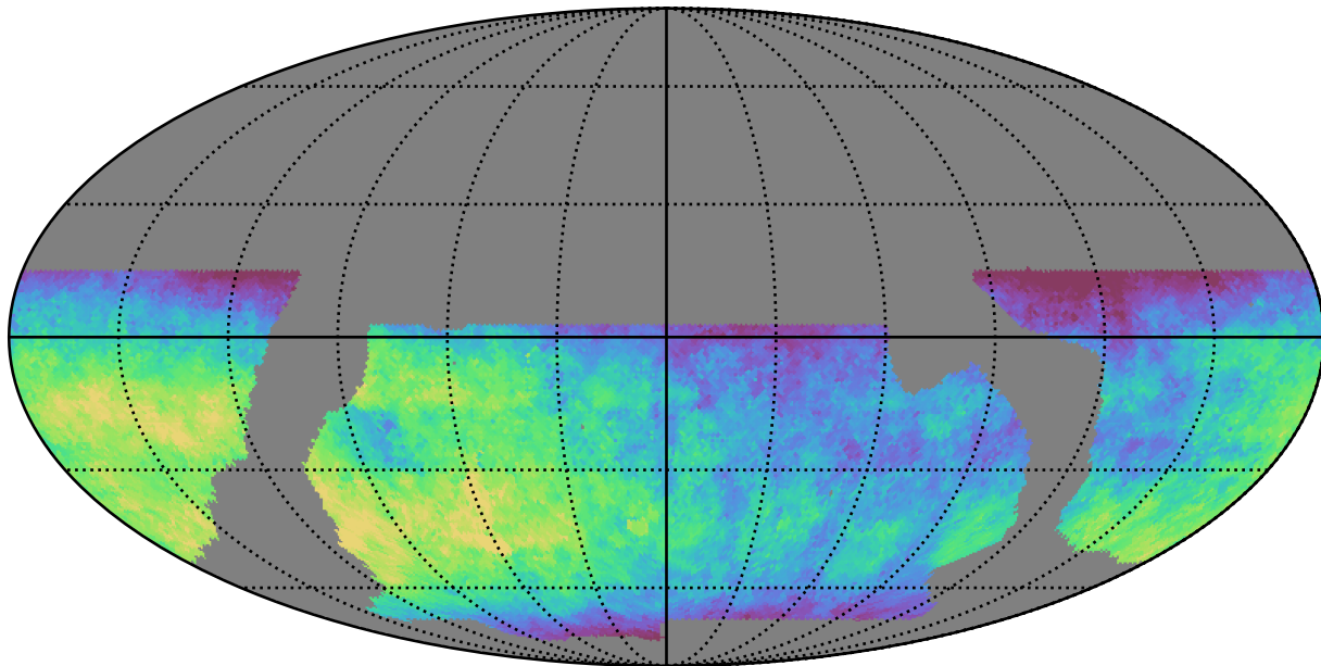
baseline_v2.0_10yrs WFD r band: Median fiveSigmaDepth
