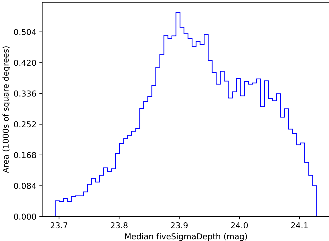
baseline_v2.0_10yrs WFD r band: Median fiveSigmaDepth
