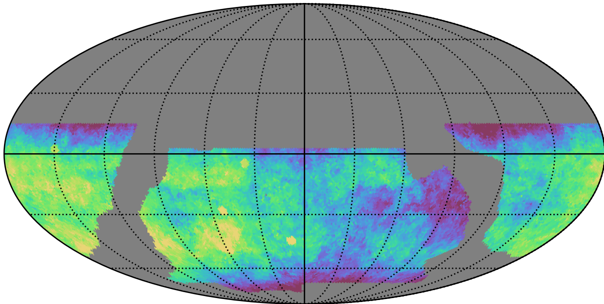
baseline_v2.0_10yrs WFD i band: Median fiveSigmaDepth
