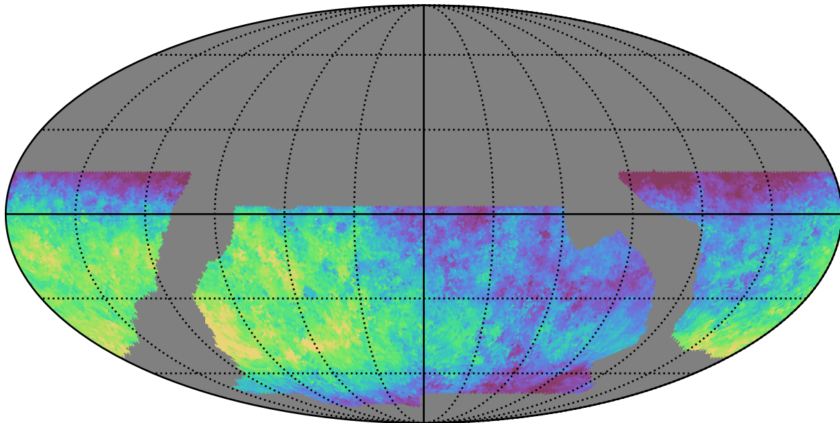
baseline_v2.0_10yrs WFD g band: Median fiveSigmaDepth
