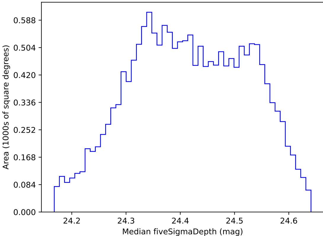
baseline_v2.0_10yrs WFD g band: Median fiveSigmaDepth
