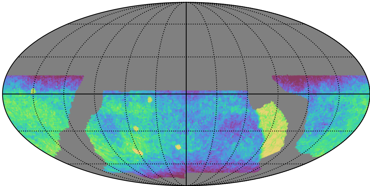
baseline_v2.0_10yrs WFD all bands: Median fiveSigmaDepth
