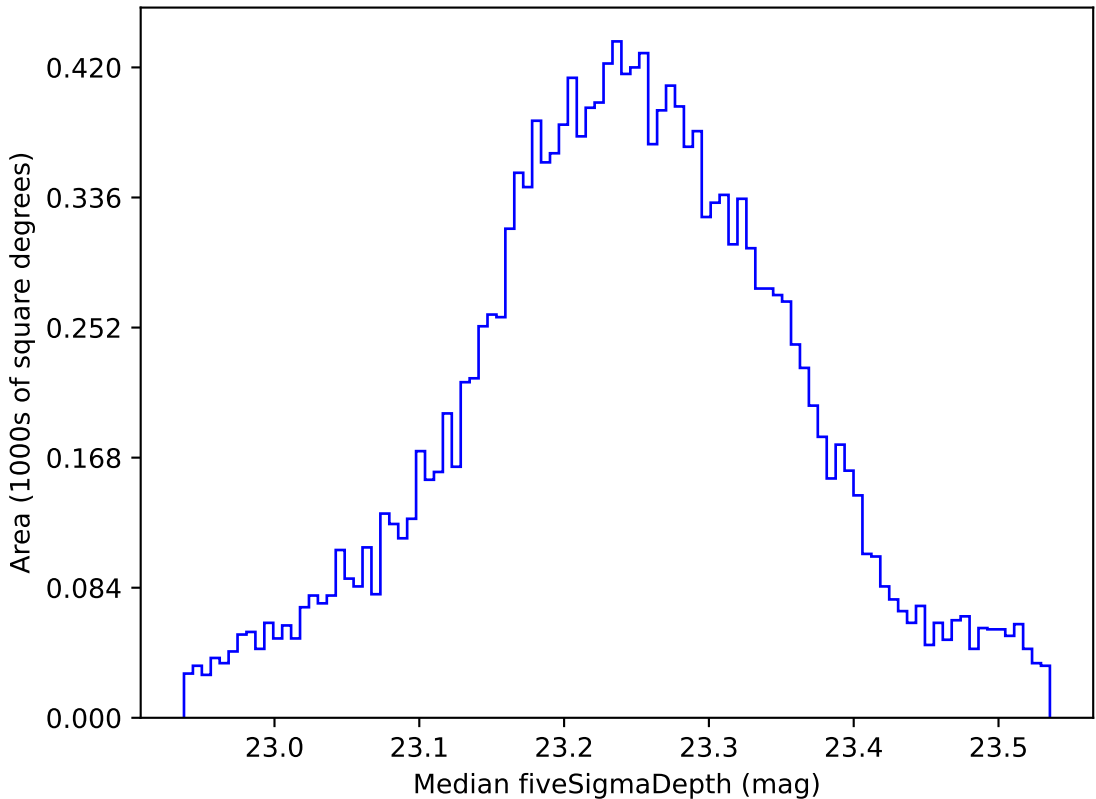
baseline_v2.0_10yrs WFD all bands: Median fiveSigmaDepth
