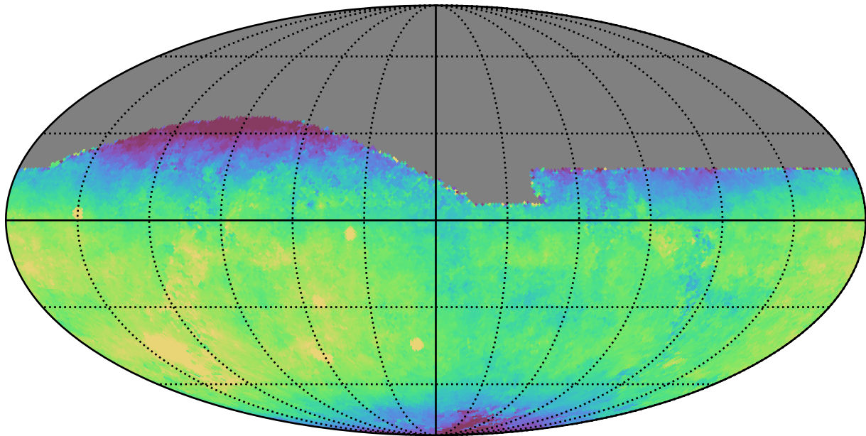
baseline_v2.0_10yrs All sky z band: Median fiveSigmaDepth
