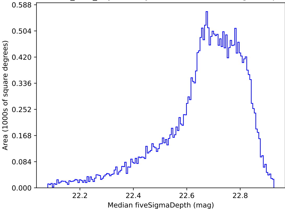
baseline_v2.0_10yrs All sky z band: Median fiveSigmaDepth
