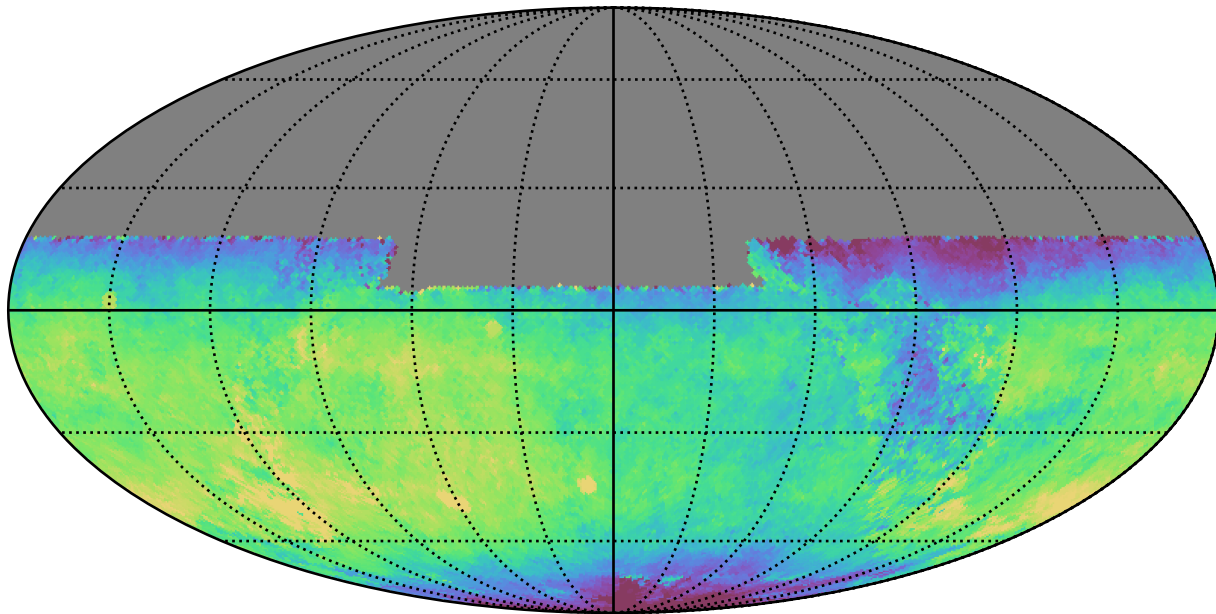
baseline_v2.0_10yrs All sky y band: Median fiveSigmaDepth
