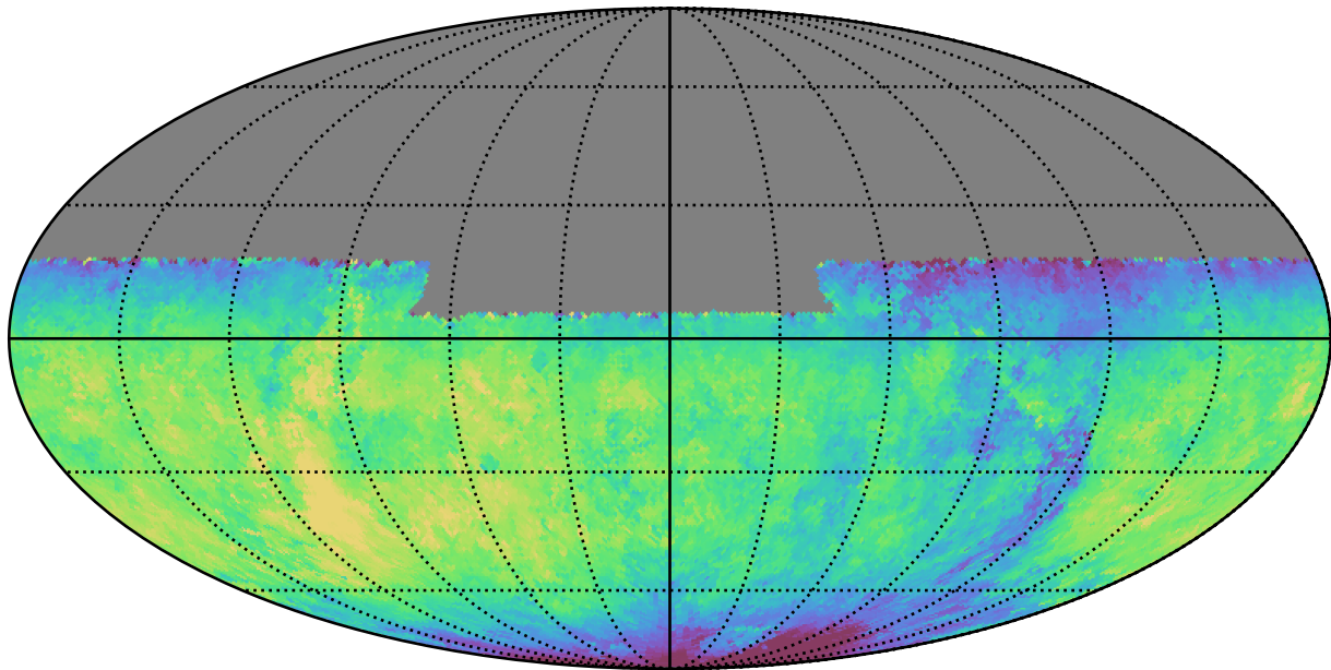
baseline_v2.0_10yrs All sky u band: Median fiveSigmaDepth
