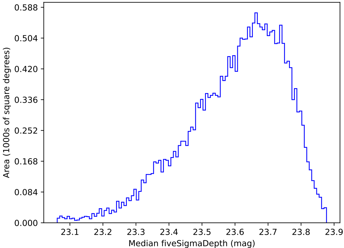
baseline_v2.0_10yrs All sky u band: Median fiveSigmaDepth
