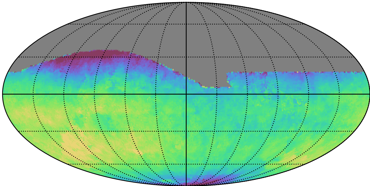
baseline_v2.0_10yrs All sky r band: Median fiveSigmaDepth
