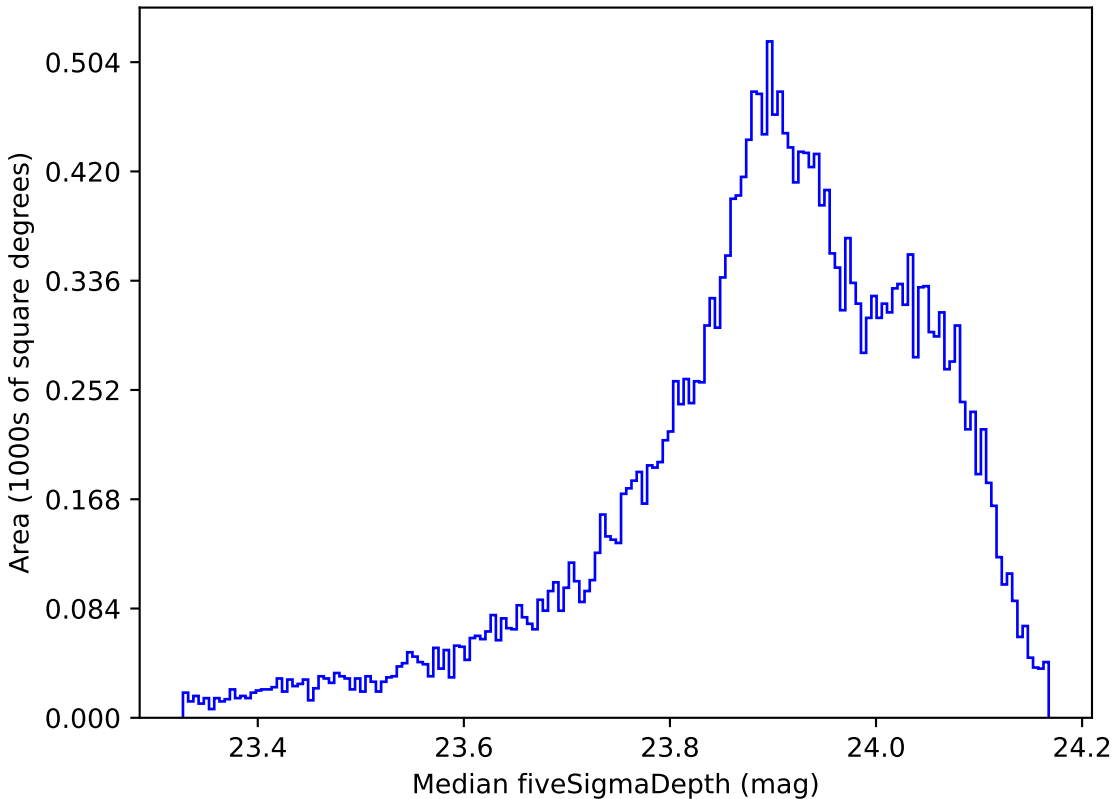
baseline_v2.0_10yrs All sky r band: Median fiveSigmaDepth
