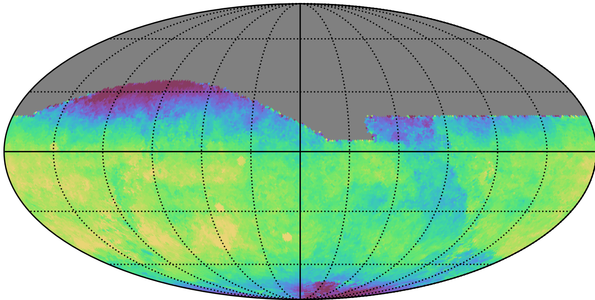
baseline_v2.0_10yrs All sky i band: Median fiveSigmaDepth
