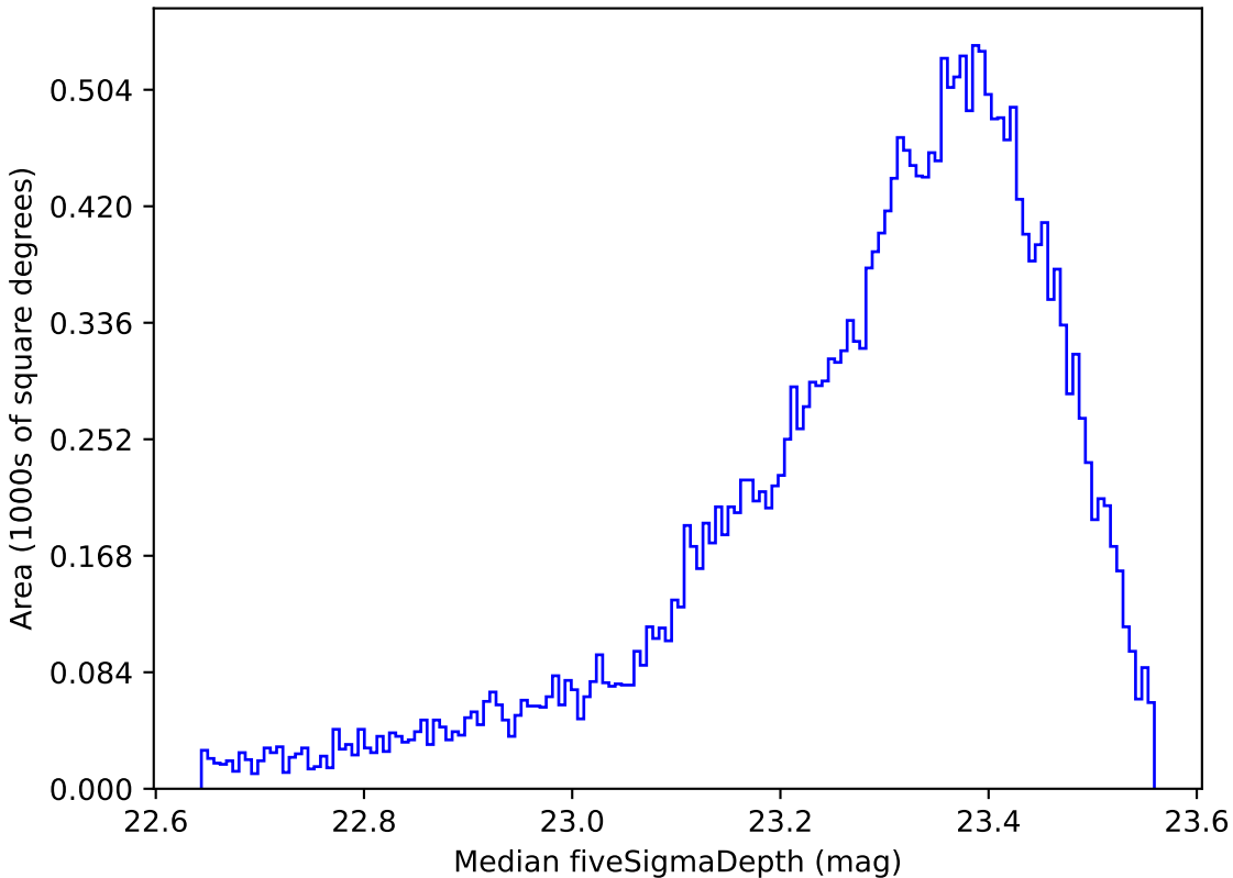
baseline_v2.0_10yrs All sky i band: Median fiveSigmaDepth
