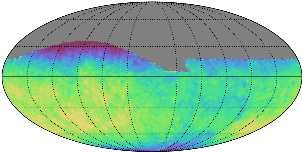
baseline_v2.0_10yrs All sky g band: Median fiveSigmaDepth
