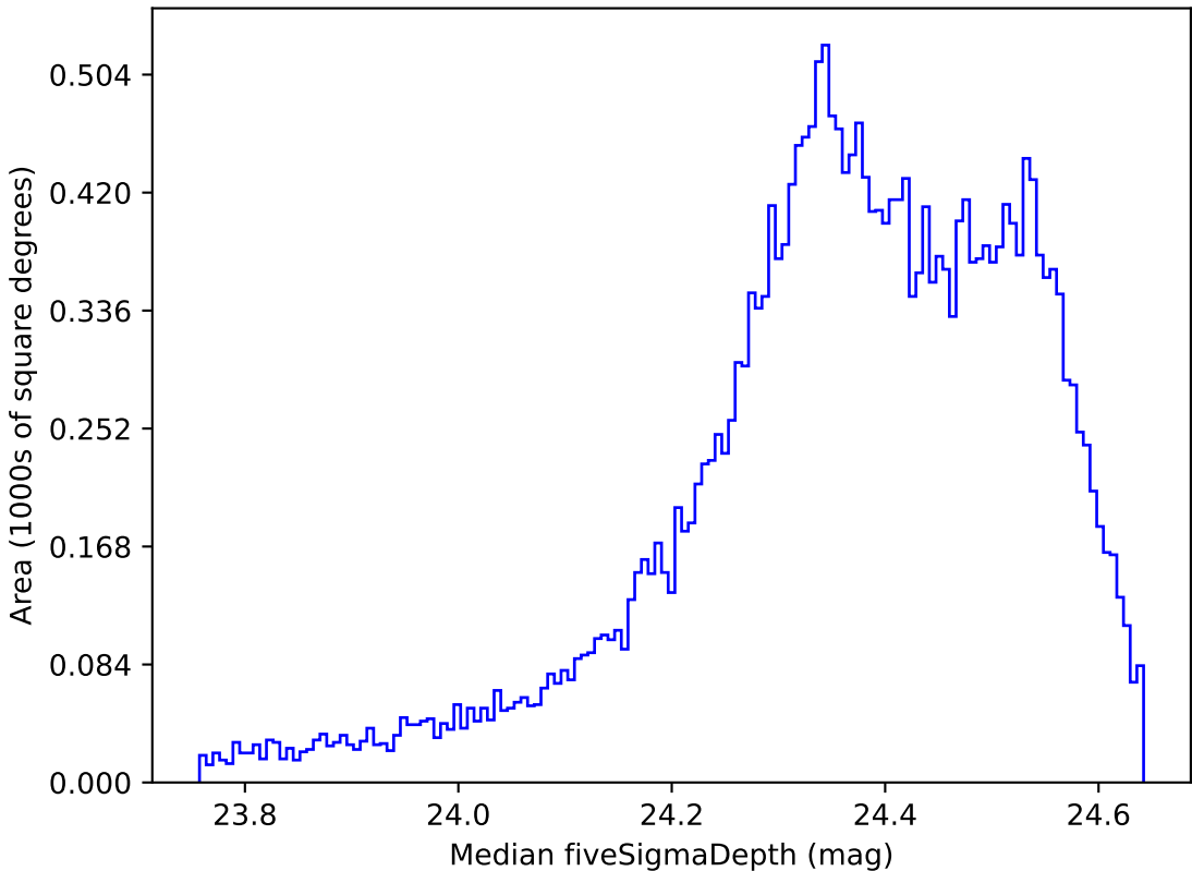
baseline_v2.0_10yrs All sky g band: Median fiveSigmaDepth
