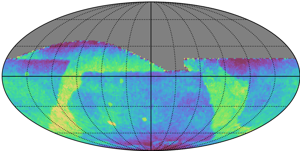
baseline_v2.0_10yrs All sky all bands: Median fiveSigmaDepth
