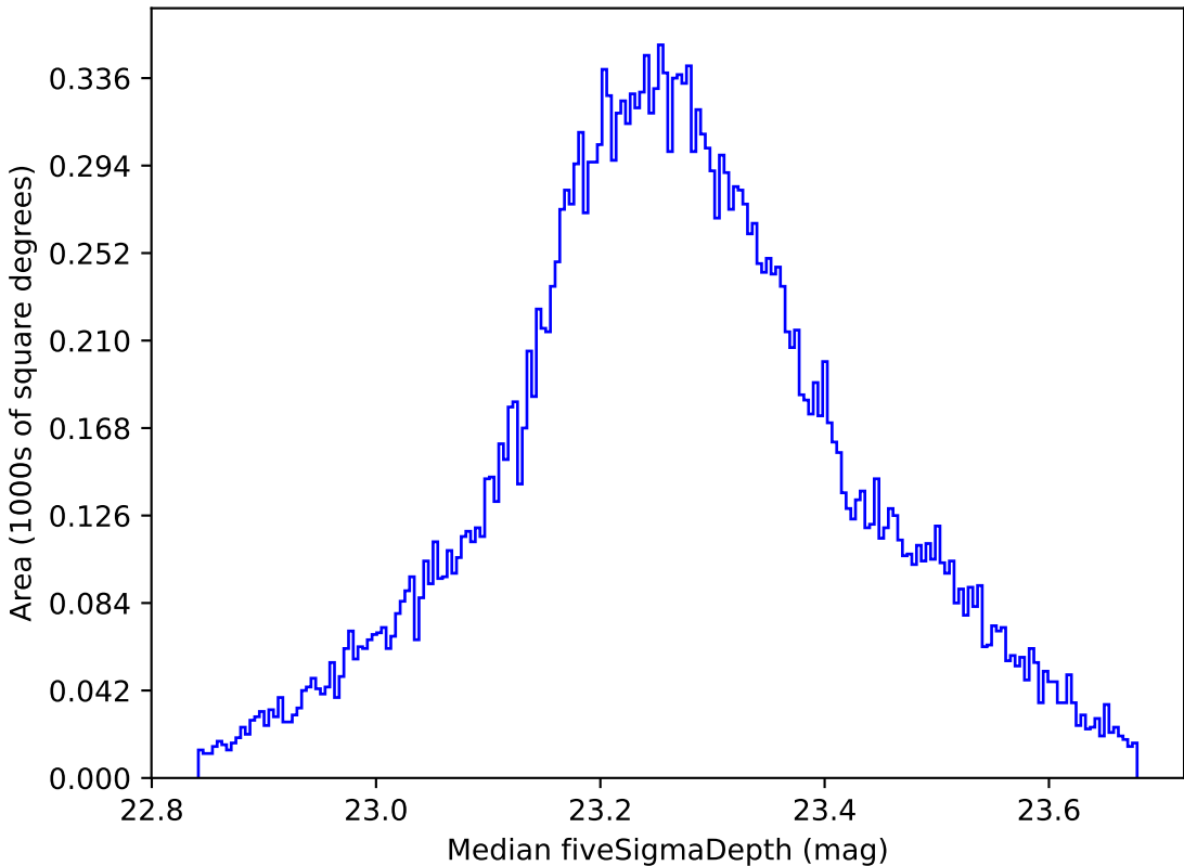
baseline_v2.0_10yrs All sky all bands: Median fiveSigmaDepth
