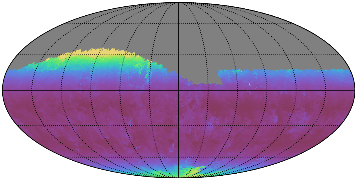
baseline_v2.0_10yrs Yr 1 z band: Median airmass
