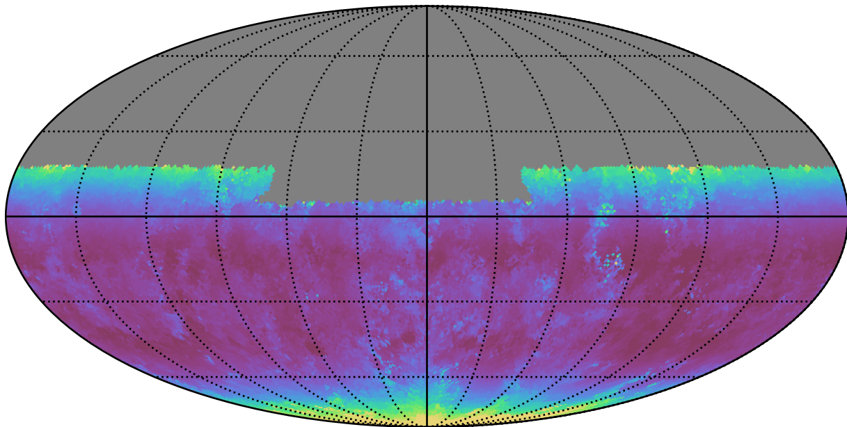
baseline_v2.0_10yrs Yr 1 y band: Median airmass
