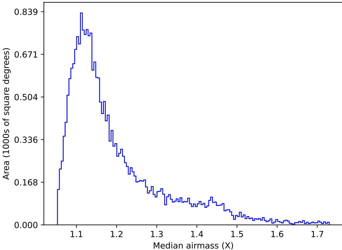
baseline_v2.0_10yrs Yr 1 y band: Median airmass
