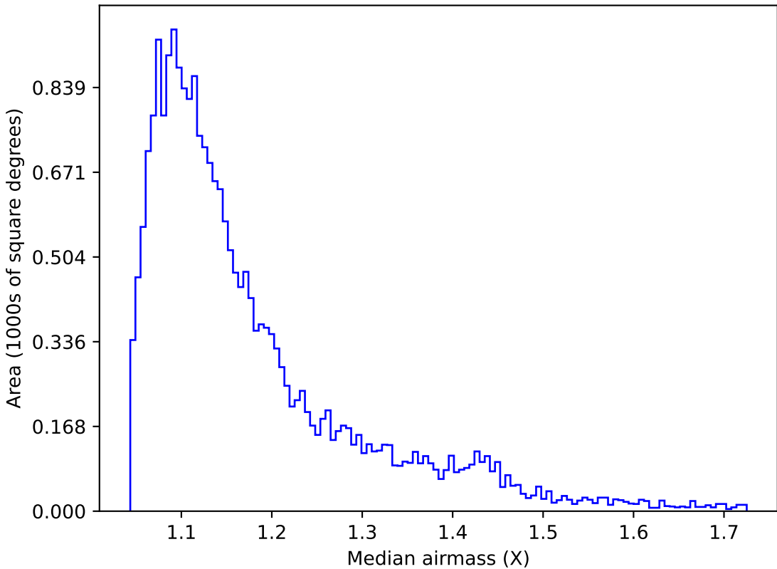
baseline_v2.0_10yrs Yr 1 u band: Median airmass
