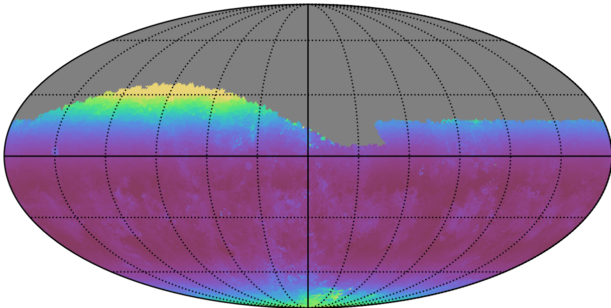
baseline_v2.0_10yrs Yr 1 r band: Median airmass
