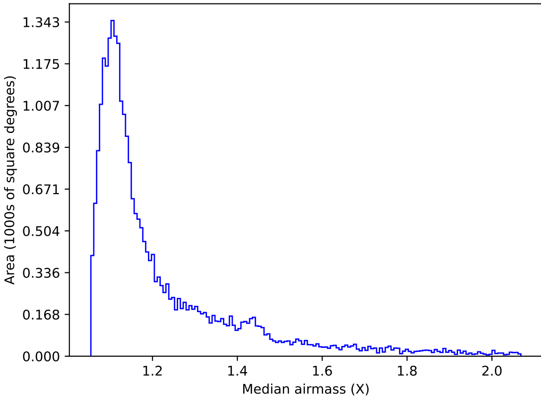
baseline_v2.0_10yrs Yr 1 r band: Median airmass
