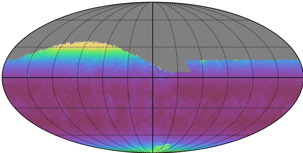
baseline_v2.0_10yrs Yr 1 i band: Median airmass
