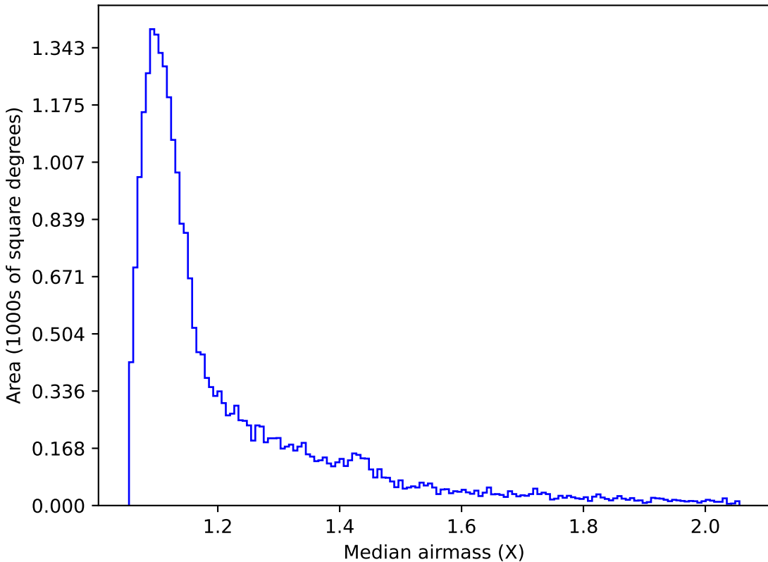
baseline_v2.0_10yrs Yr 1 i band: Median airmass
