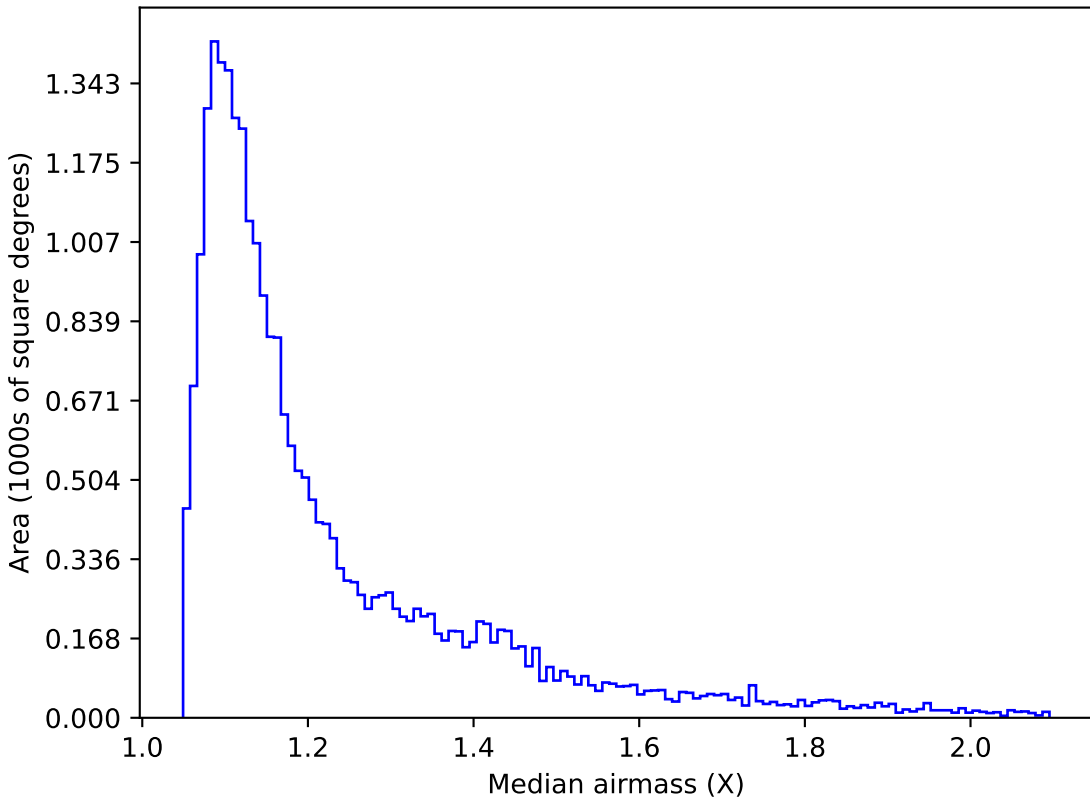
baseline_v2.0_10yrs Yr 1 g band: Median airmass
