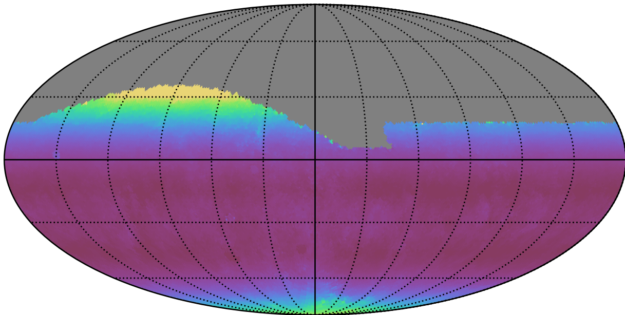
baseline_v2.0_10yrs Yr 1 all bands: Median airmass
