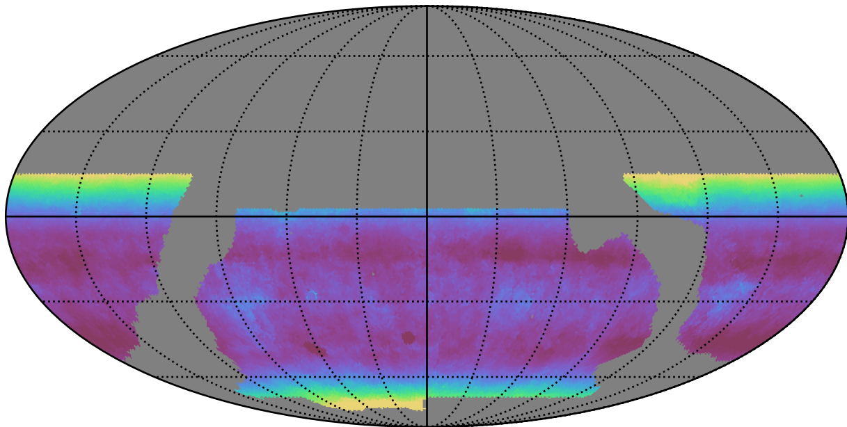
baseline_v2.0_10yrs WFD z band: Median airmass
